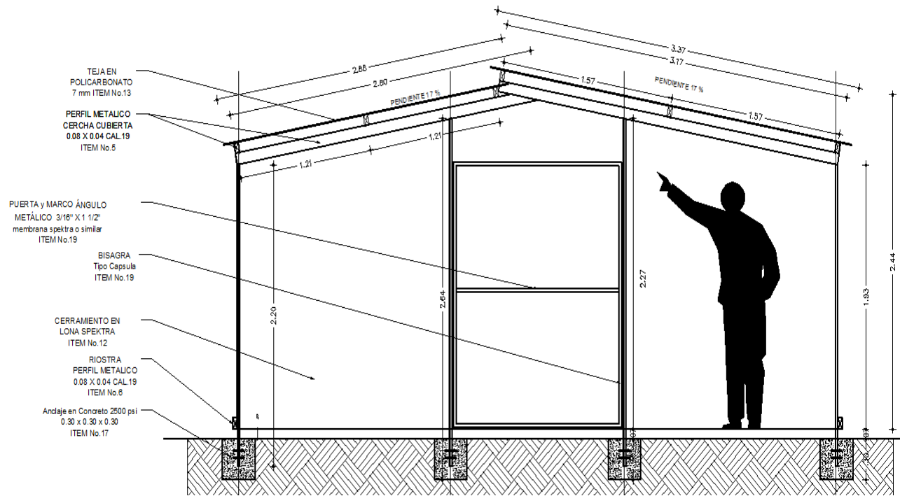
PLANO No.9 – PLANO FACHADA FRONTAL
