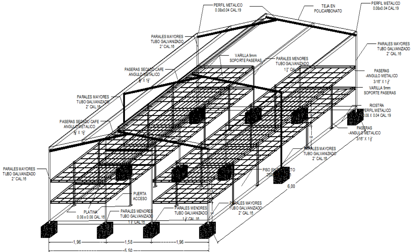
PLANO No.1 – PLANTA GENERAL SECADERO
